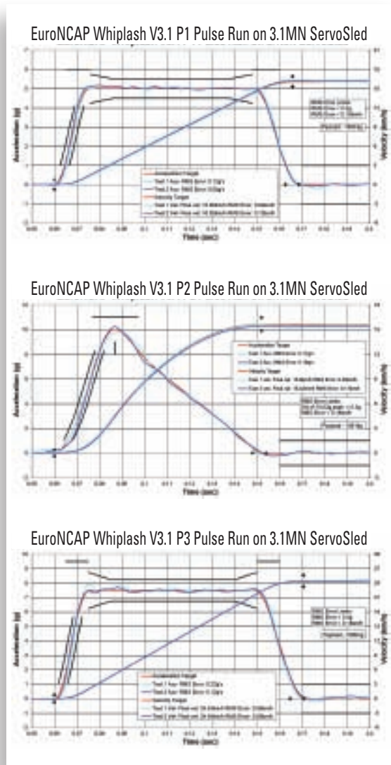
Whiplash test program with repeatable pulses within corridors.
