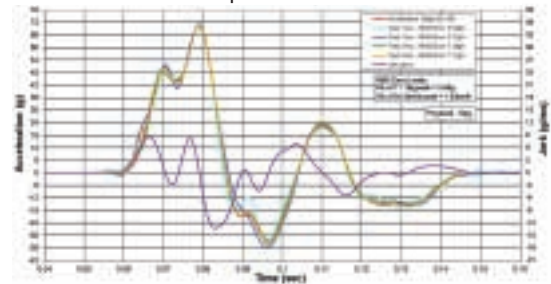
ServoSled - Side Impact Pulse
